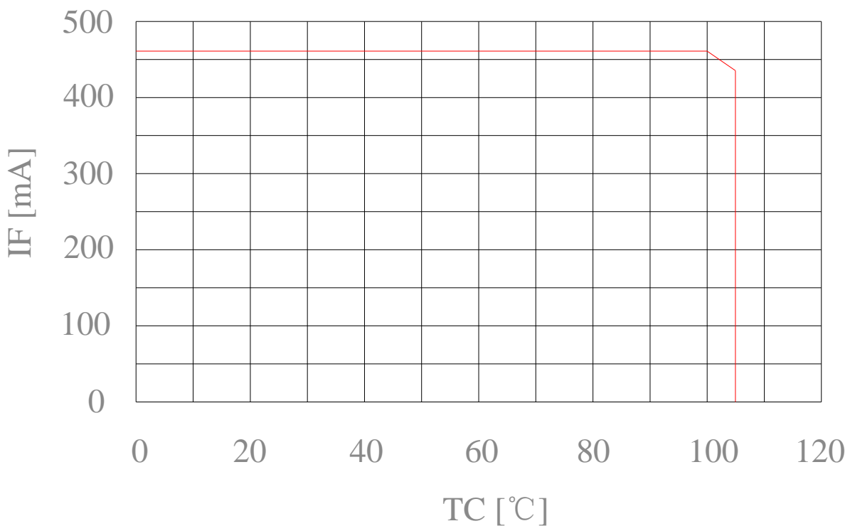
Case Temperature VS. Allowable Forward Current
